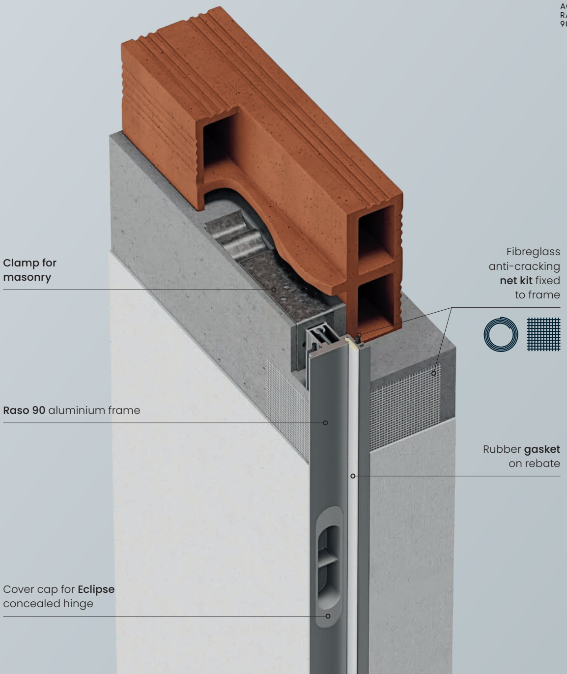
PUSH APPLICATION
