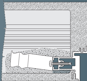
PULL APPLICATION
