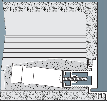
PUSH APPLICATION
