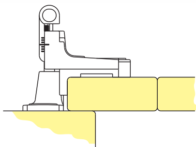
Overlapped closure
